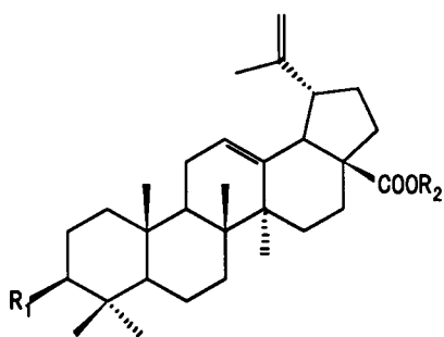
Cirensenoside P (22)
