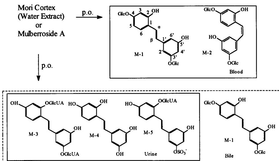
Fig. 1. Absorption and Metabolism of Mulberroside A M-1: mulberroside A, M-2: cis-mulberroside A, M-3: oxyresveratrol 2,3'-di-o- \beta -D-glucuronide M-4: oxyresveratrol , M-5: oxyresveratrol 2-O- \beta -glucuronide-3'-O-sulfate
