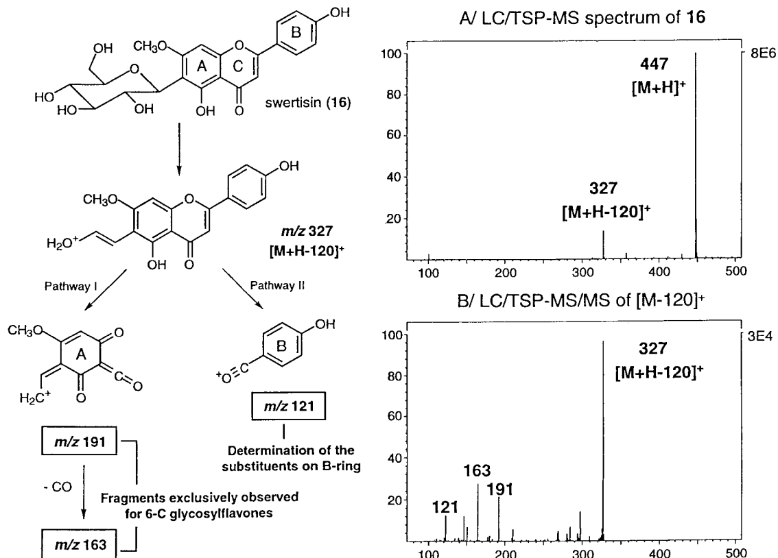
Fig. 10. LC/TSP-MS (a) and LC/TSP-MS/MS (b) spectra of swertisin ( 16 ) in the crude extract of G. ottonis . The LC/MS/MS analysis was performed using the fragment [M+H-120]^+ (spectrum a) as parent ion. Characteristic daughter ions at m/z 121, 163 and 191 were observed, indicating the substitution on the A- and B-ring of the C-glycosylflavone 16 .
