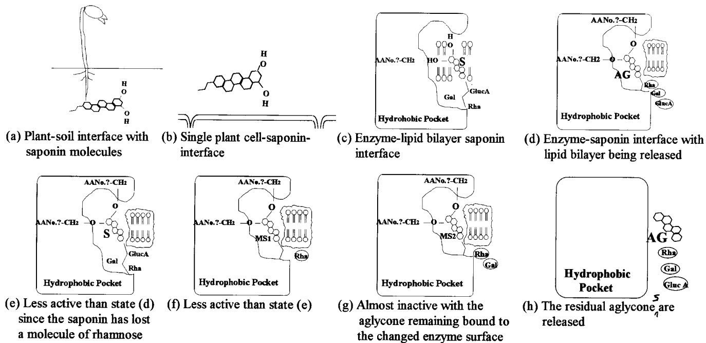
Figure 14. Suggested mechanism of action of mono- and bidesmoside saponins that occur in mungbeans used as an addition to water in the growth of mungbeans and lettuce in a 72-h bioassay. Note: Sugars from soyasaponin I were used as an example; which amino acid number is not known for co-valent binding; S = saponin; MS1 = saponin without one molecule of sugar; MS2 = saponin with loss of two molecules of sugar; AG = aglycone with rhamnose, galactose and glucuronic acid free in the medium.
