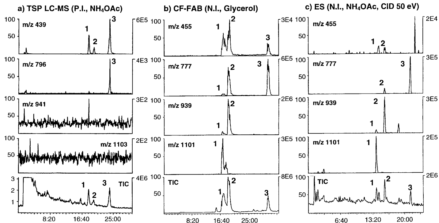
Fig. 4. Combined LC/TSP-MS, LC/CF-FAB-MS and LC/ES-MS of the MeOH extract of Swartzia madagascariensis (Leguminosae). HPLC: C18 Nova-Pak (4 \mu m, 150 x 3.9 mm i.d.); gradient, CH 3 CN-H 2 O (0.05% TFA) 30:70 ->50:50 in 30 min (0.9 ml/min)
