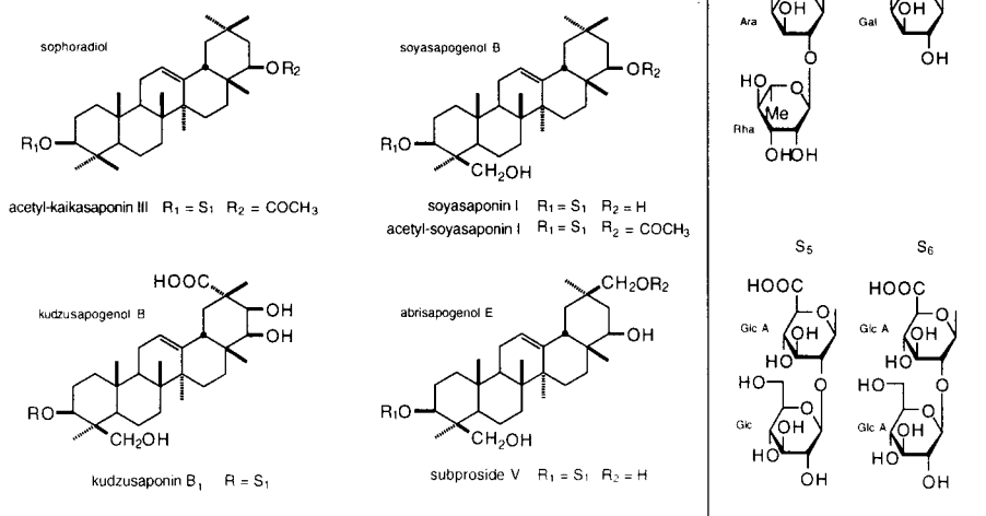
Fig. 3.2. Oleanene Glycosides from Puerariae Thomsonii Radix
