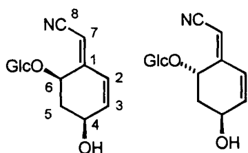
menisdaurin (1) [lit. 8-13, 15, 20]
