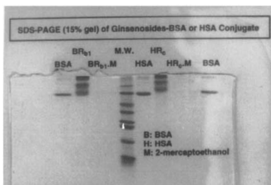
Fig. 4. Gel electrophoretogram(PAGE 15%) of ginsenoside-protein conjugates.
