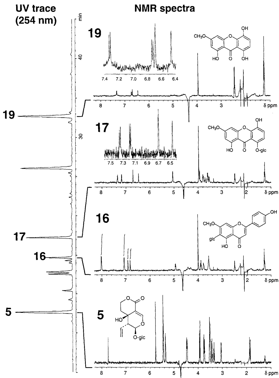
Fig. 9. LC/UV chromatogram of G. ottonis (vertical display) with the stop-flow LC/ ^1\text{H} -NMR spectra of 5, 16, 17 and 19. On these LC/ ^1\text{H} -NMR spectra, the coupling constants and the integration of the aromatic signals were easily measured.
