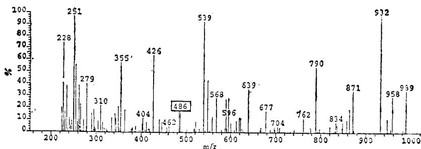
Fig. 4 Linked- scanning FAB-MS spectrum of oligosaccharide DP-6
