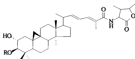
mussaendoside
