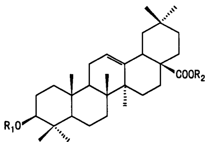
Elatoside A (23)
