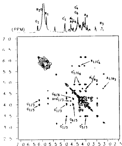
Figure 6 NOESY spectrum of 1 at 2 °C; intrasidue NOE's of sugars are labelled under diagonal and interresidue NOE's are above diagonal. At rt, the NOE between Ara'.H 1 and Ara'.H 2 was not observed.
