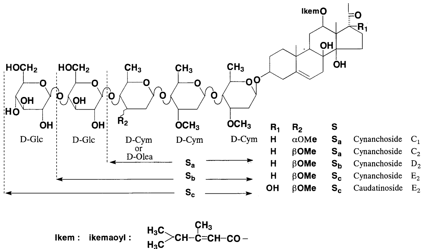
Chart 2 Glycosides isolated from the root of Cynanchum caudatum (牛皮消根)
