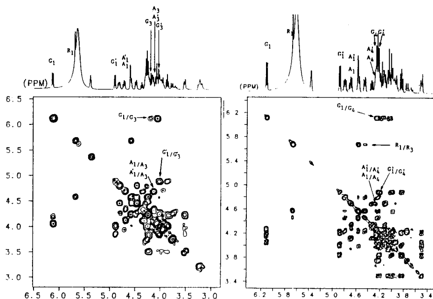
Figure 2 (a) Single RCT spectrum of 1. Labelled peaks indicate the relayed coherence transfers between anomeric protons of sugar residues with their respective 3-position protons. (b) Double RCT spectrum of 1. Labelled peaks indicate the relayed coherence transfers between anomeric protons with their respective 4-position protons, and the coherence transfer between Rha.H 1 with Rha.H 3 .
