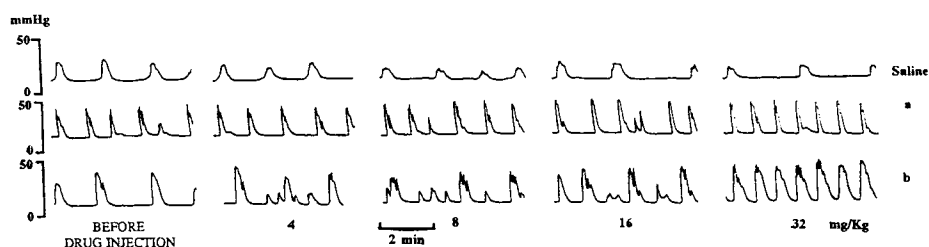
Figure 1. Typical traces of the effects of intravenous injection (a) or intrauterine injection (b) of 3 on spontaneous uterine contractility of anesthetized rats in vivo . Each episode shows only a few minutes of the maximal activity of each dose of 3.
