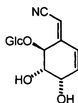
dasycarponin (5) [lit. 14, 15]
