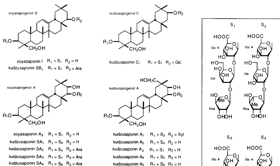
Fig. 3.1. Oleanene Glycosides from Puerariae Lobata Radix
