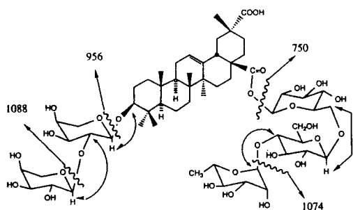
Figure 4. Mass spectral fragmentations and interglycosidic NOE's of 1 for sugar sequence and linkage site determination.
