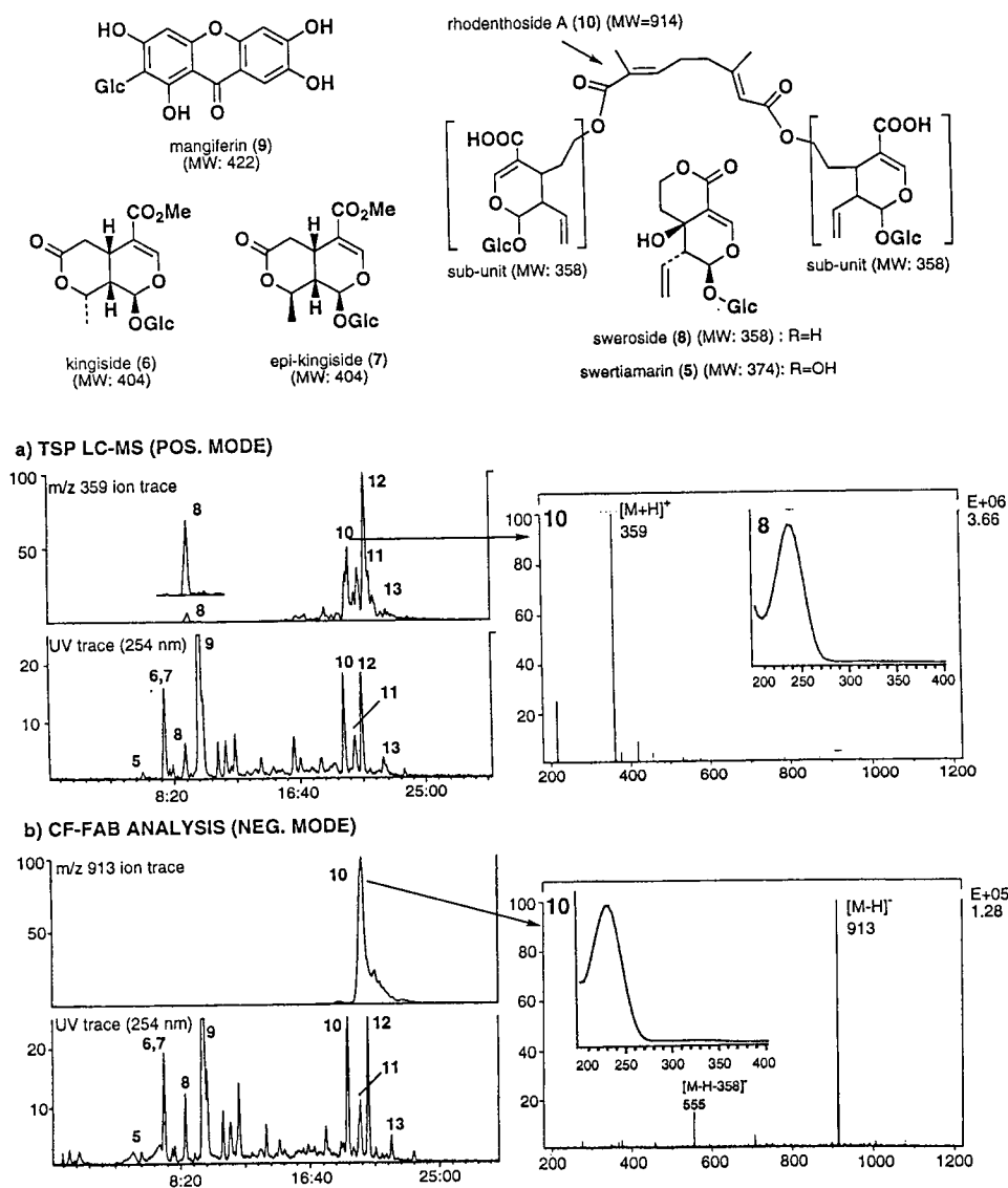
Fig. 7. Combined TSP (a) and CF-FAB (b) LC/MS of the enriched BuOH fraction of the methanolic extract of Gentiana rhodantha (Gentianaceae). HPLC: Column, RP-18 NovaPak (4 \mu m, 150 x 3.9 mm i.d.); gradient, CH 3 CN-H 2 O (0.05% TFA) 5:95 \rightarrow 50:50 in 30 min (0.9 ml/min). TSP (a): Positive ion mode; filament off; vaporiser, 90°C; source, 230°C; AcONH 4 0.5 M (0.2 ml/min post-column). CF-FAB (b): Negative ion mode; FAB tip 50°C; source 100°C; glycerol 50% (v/v) (0.15 ml/min post-column); LC flow post column split 1:100.
