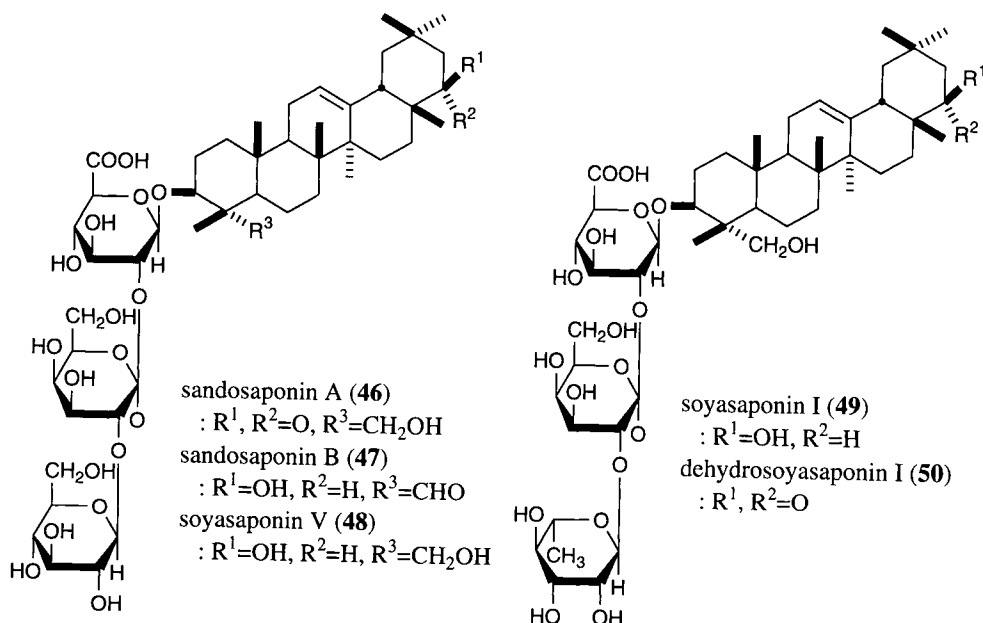
Chart 9. Structure of Saponin constituents from Kidney Bean
