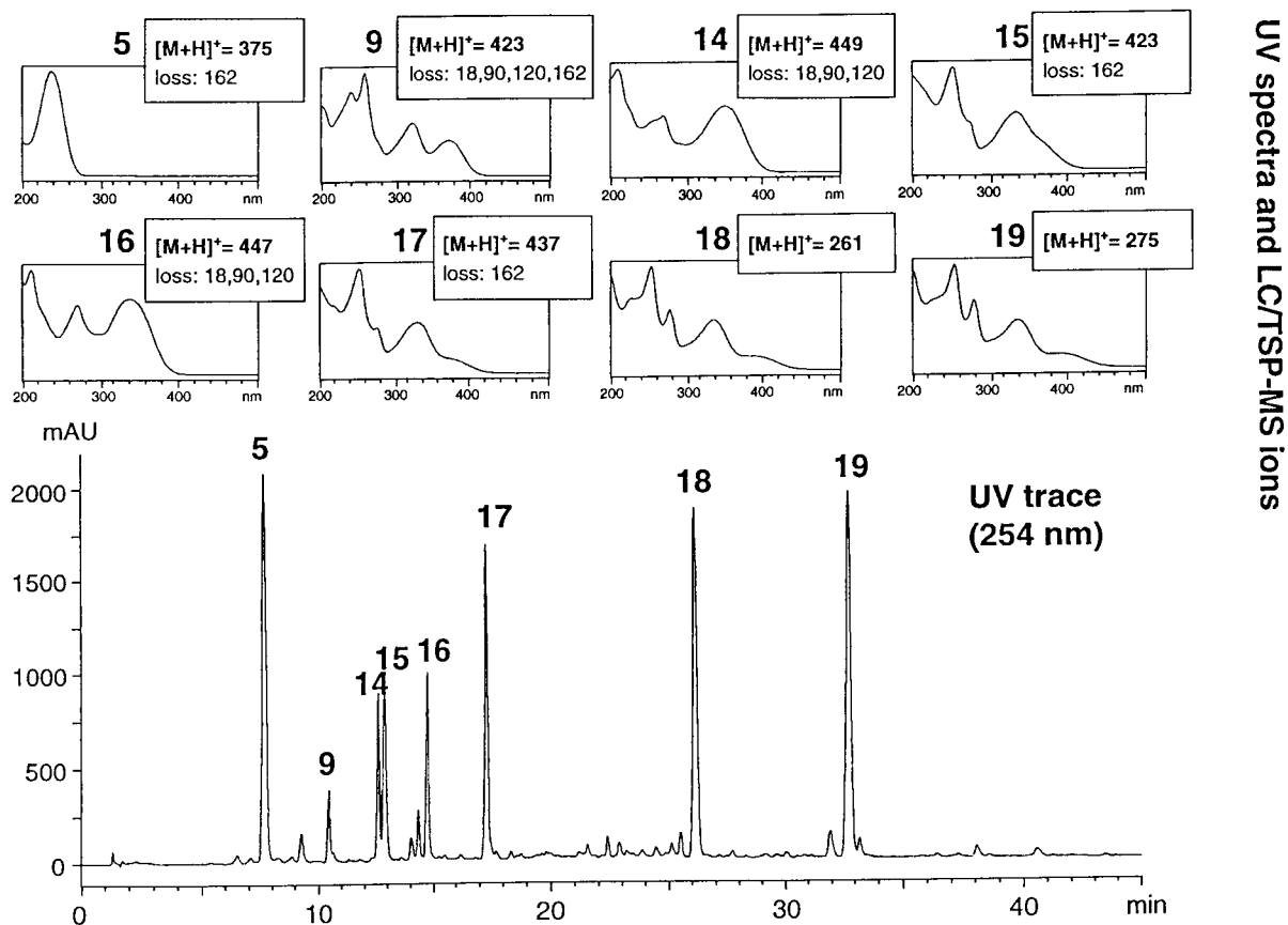
Fig. 8. LC/UV chromatogram of G. ottonis with UV spectra and main FSP/LC-MS ions of the major constituents. HPLC: Column, RP-18 NovaPak (4 \mu m, 150 x 3.9 mm i.d.); gradient, CH 3 CN-H 2 O (0.05% TFA) 5:95 \rightarrow 65:35 in 50 min (1.0 ml/min). UV spectra of 14 and 16 were characteristic for flavones, while those of 15 and 17-19 were indicative of xanthenes and those of 5 of a secoiridoid glycoside.
