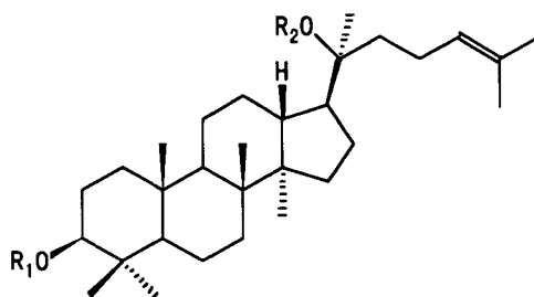
Vina-ginsenoside-R3 (5)
