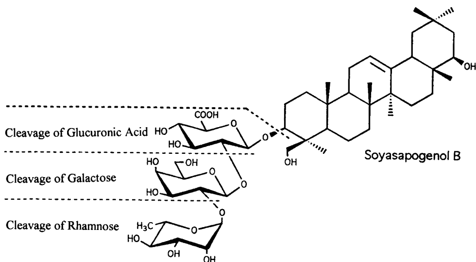
Fig. 11. Suggested structural changes in soya saponin I (3-O-[ \alpha -L-rhamnopyranosyl-(1 \rightarrow 2)- \beta -D-galactopyranosyl-(1 \rightarrow 2)- \beta -D-glucuronopyranosyl] soya sapogenol B) that occur on the mungbean root surface and in the surrounding rhizosphere. Legend: Stimulation occurs when soil is added; inhibition occurs when no soil is present (in the 72 h bioassay). Cleavage or loss of sugars can occur sequentially or by 2- or 3-piece fragments.
