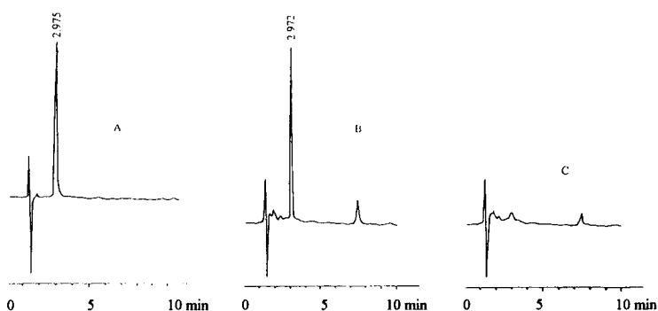
Fig. HPLC chromatograms of standard paeonflorin (A), Qinggan Injection (B) and sample without Paeonia veitchi (C).
