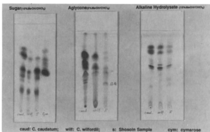
Figure 2 TLC Pattern for Sugar, Aglycone, and Alkaline hydrolysate of Aglycone of Cynanchum caudatum , C. wilfordii , and Shosoin sample
